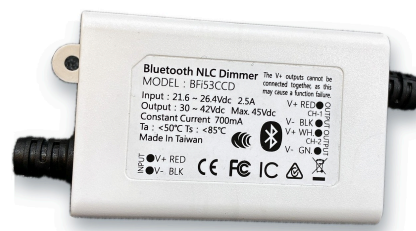
BFi53CCD, dual-channel constant-current dimmer
