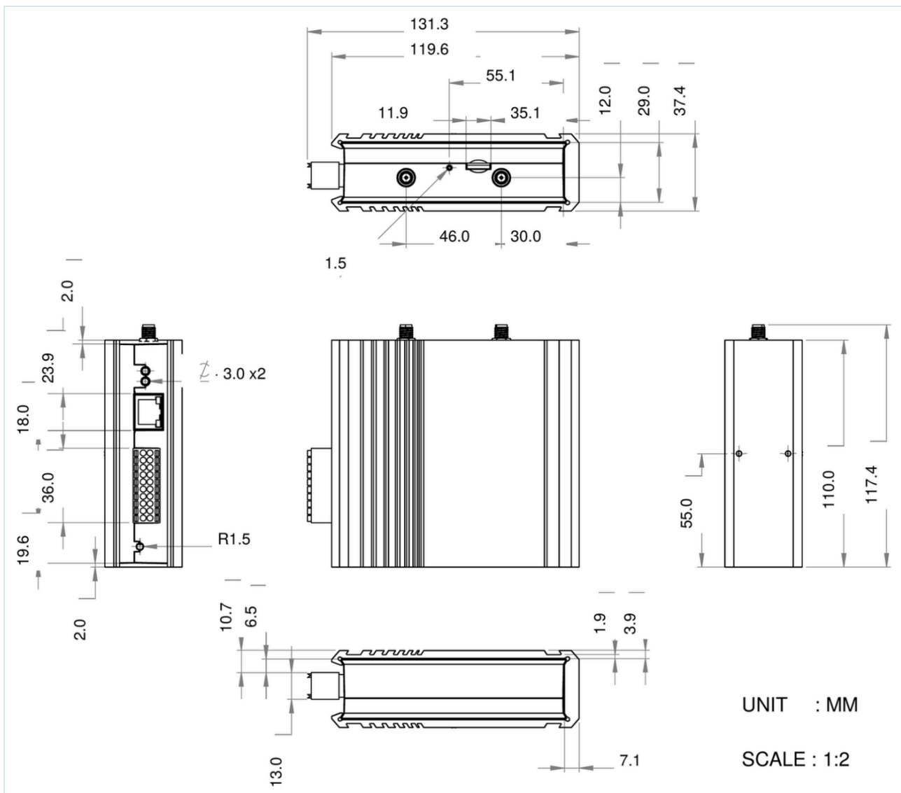
Figure 3 — Outline, millimetres, common to both models.
